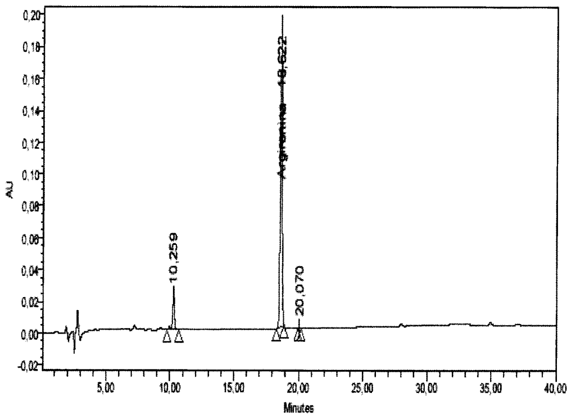
Figure 5. Chromatogram of Argireline® at initial time.
